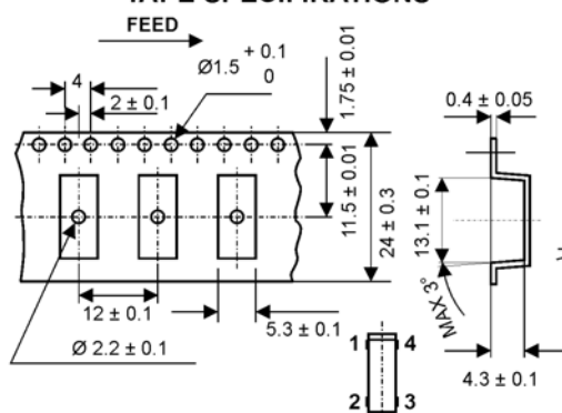
TAPE SPECIFICATIONS
