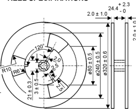
REEL SPECIFICATIONS
